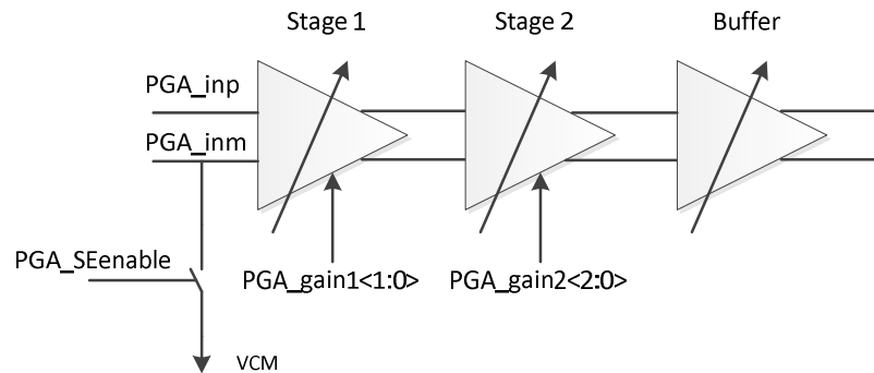
Figure 16: PGA path
