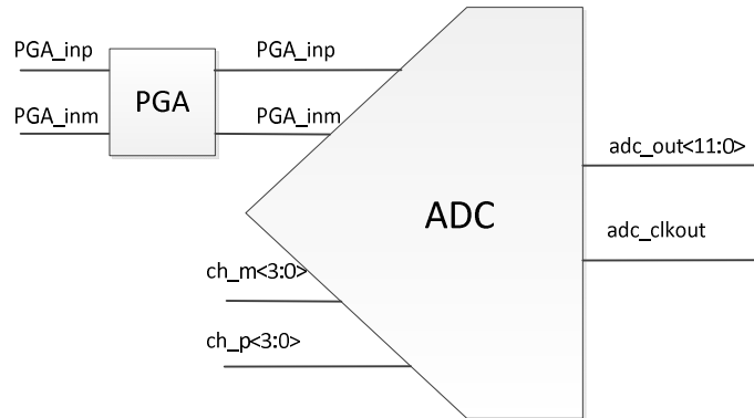
Figure 15: ADC
