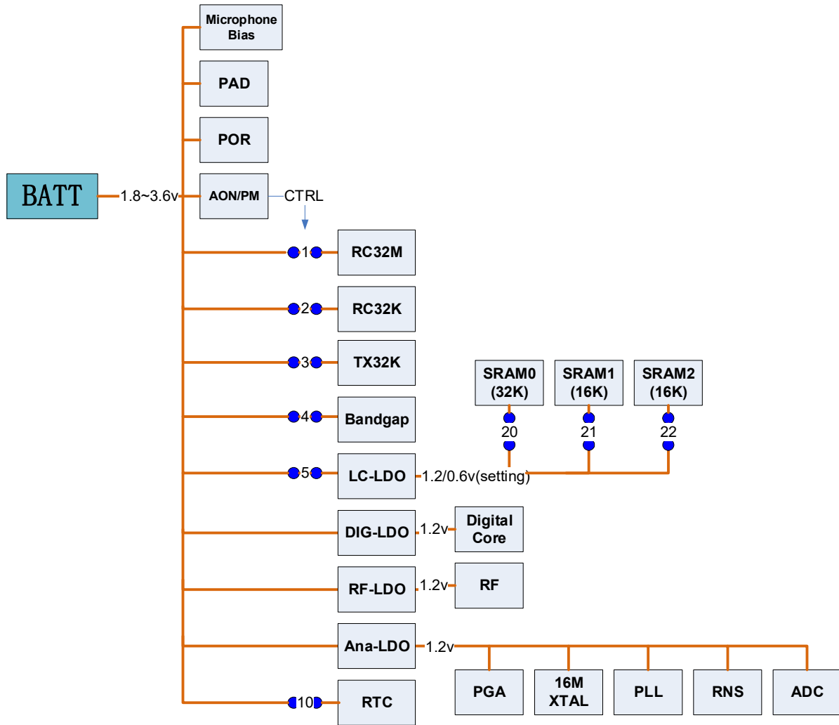
Figure 7: Power system
