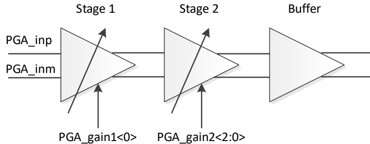
Figure 16: PGA path
