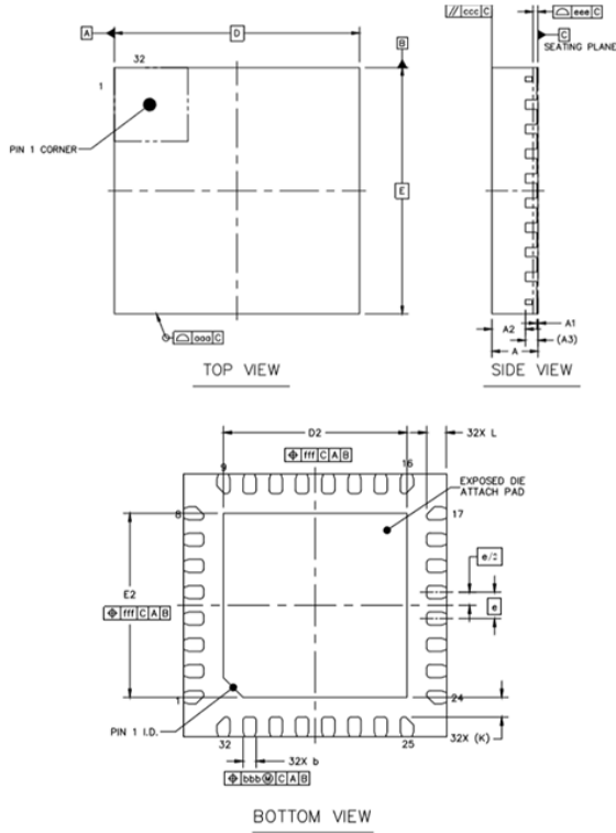
Figure 17: QFN32 package dimensions
