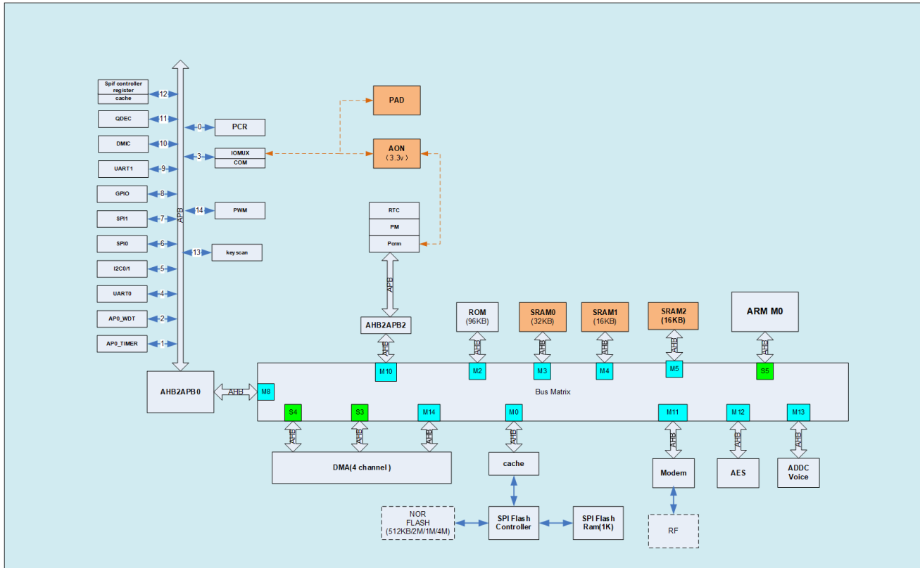
Figure 1: ST17H65 block diagram
