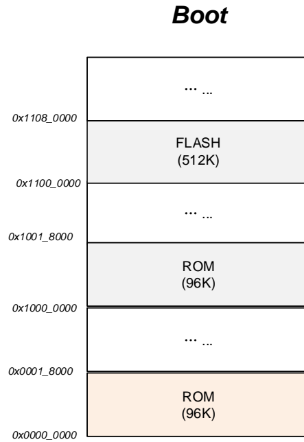
Figure 4: ST17H65 boot mode
