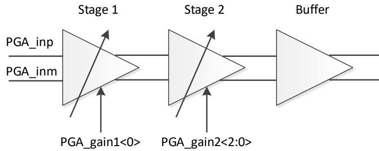
Figure 16: PGA path
