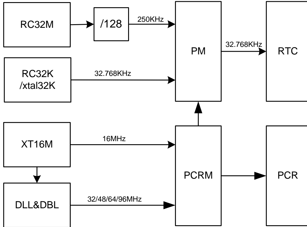
Figure 8: Clock management
